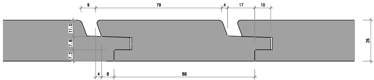
Rhomboidschalung N+K 26/88 mm
