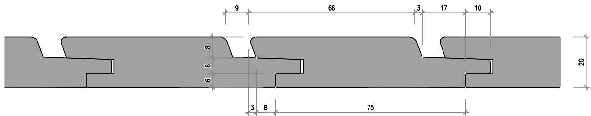
Rhomboidschalung N+K 20/75 mm
